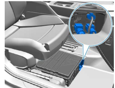
Disconnection of the 48 V vehicle electrical system for the Audi A3 Sportback.
